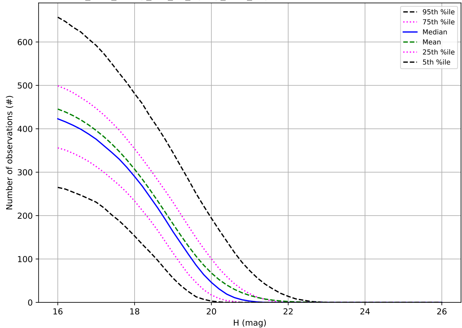
too_elab_heavy_r64_d2_ugrizy_v3.4_10yrs: Number of observations MBA
