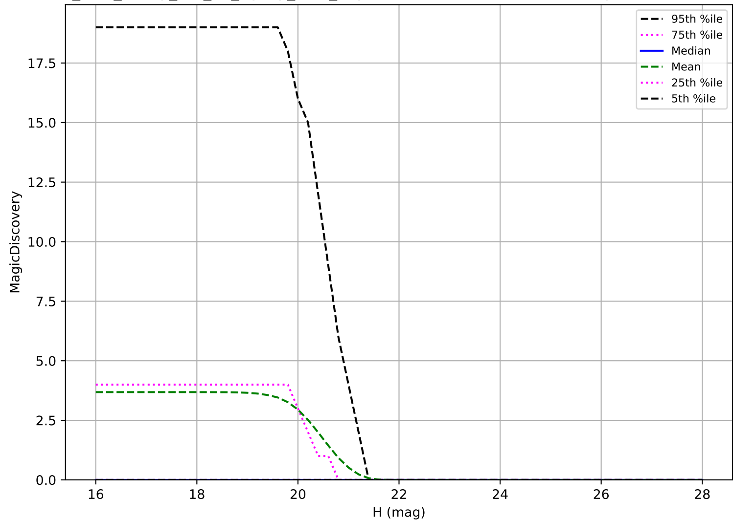
too_elab_heavy_r64_d2_ugrizy_v3.4_10yrs: Vatira 6 detections in 60 nights detection loss
