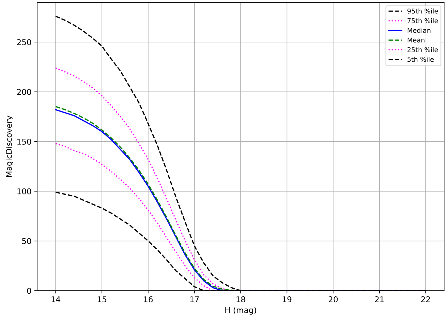
too_elab_heavy_r64_d2_ugrizy_v3.4_10yrs: Trojan 6 detections in 60 nights detection loss
