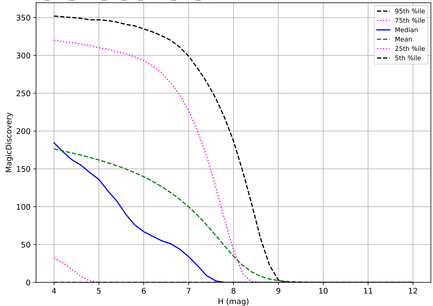
too_elab_heavy_r64_d2_ugrizy_v3.4_10yrs: TNO 6 detections in 60 nights detection loss
