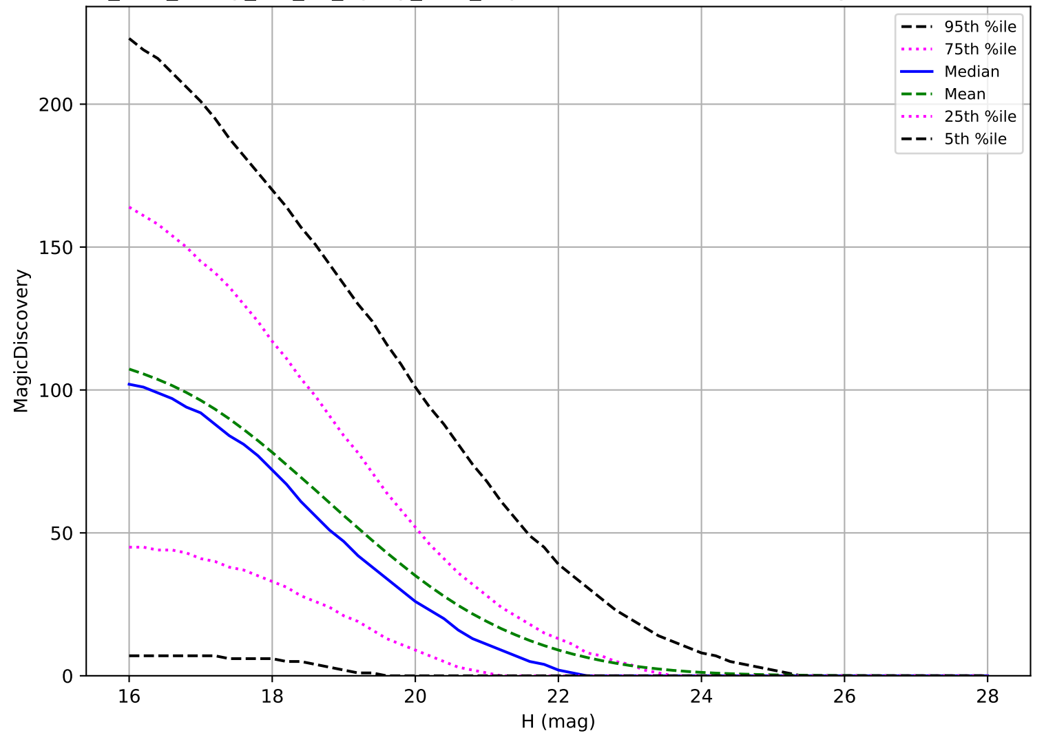
too_elab_heavy_r64_d2_ugrizy_v3.4_10yrs: PHA 6 detections in 60 nights detection loss
