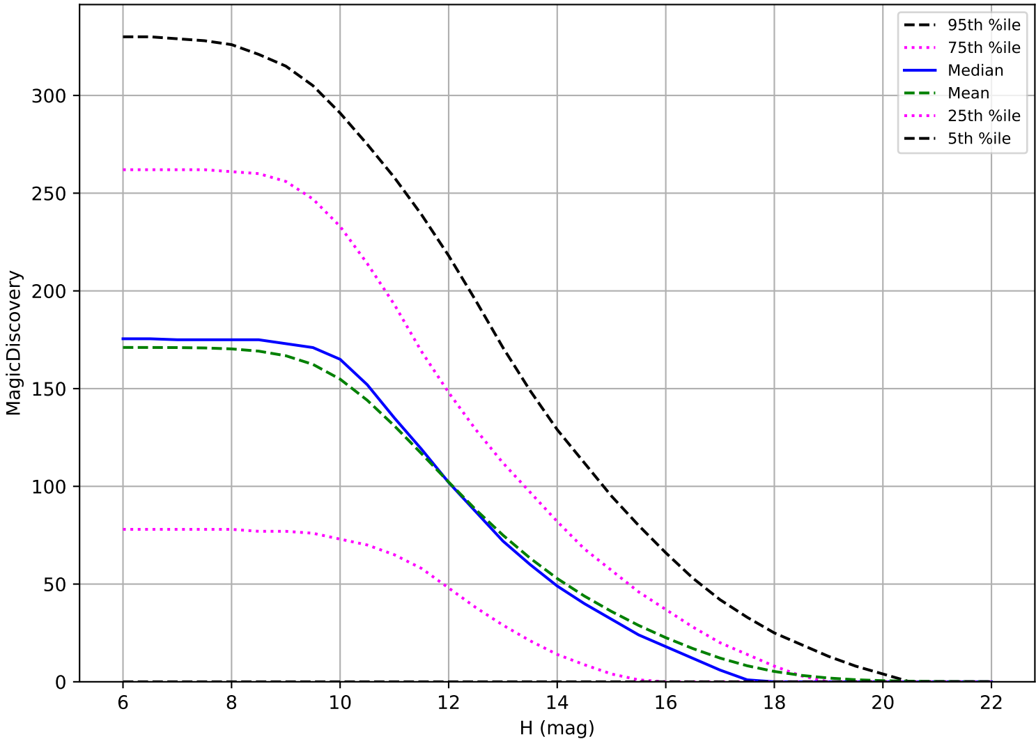
too_elab_heavy_r64_d2_ugrizy_v3.4_10yrs: OCC_r5 6 detections in 60 nights detection loss
