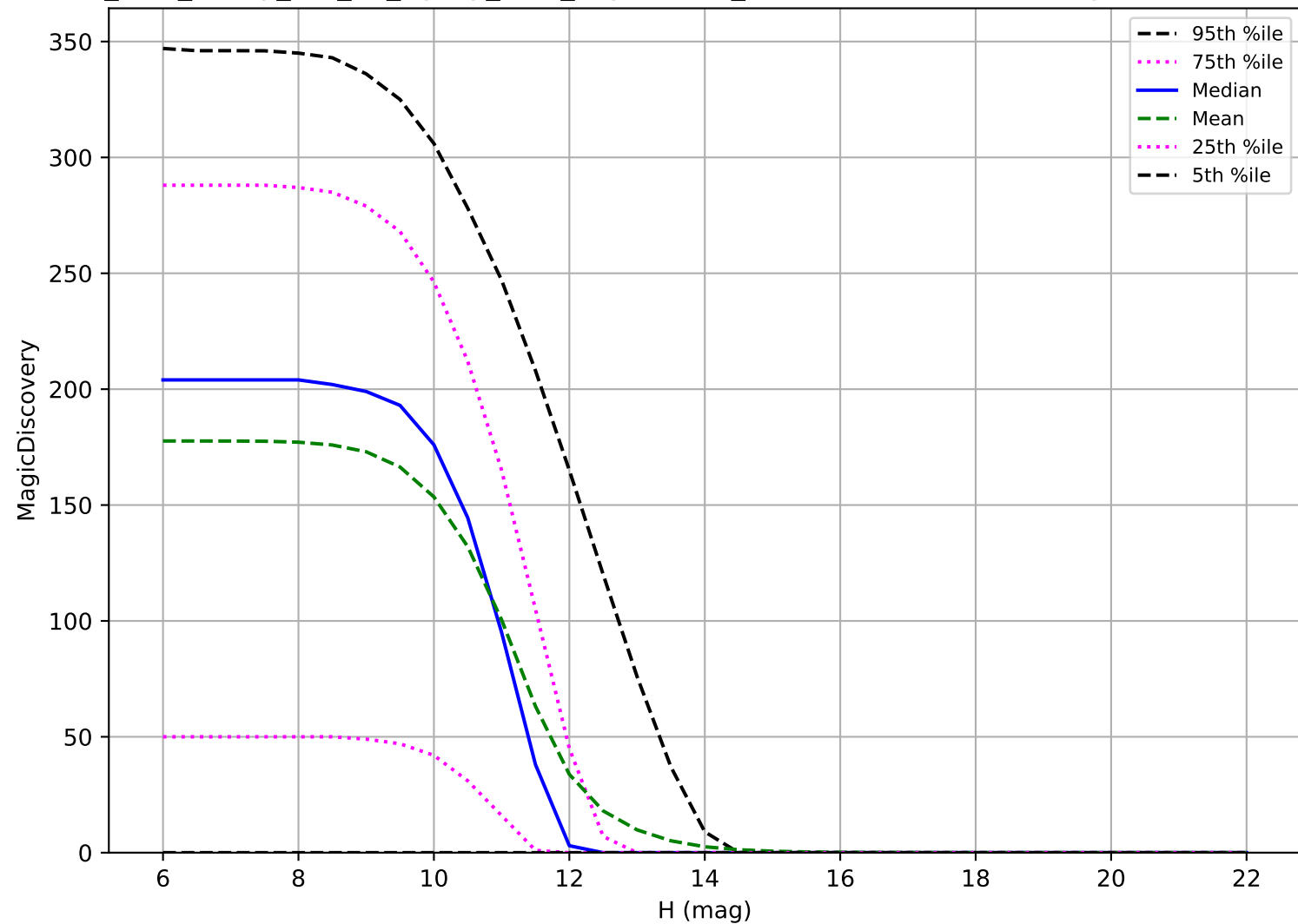
too_elab_heavy_r64_d2_ugrizy_v3.4_10yrs: OCC_r20 6 detections in 60 nights detection loss
