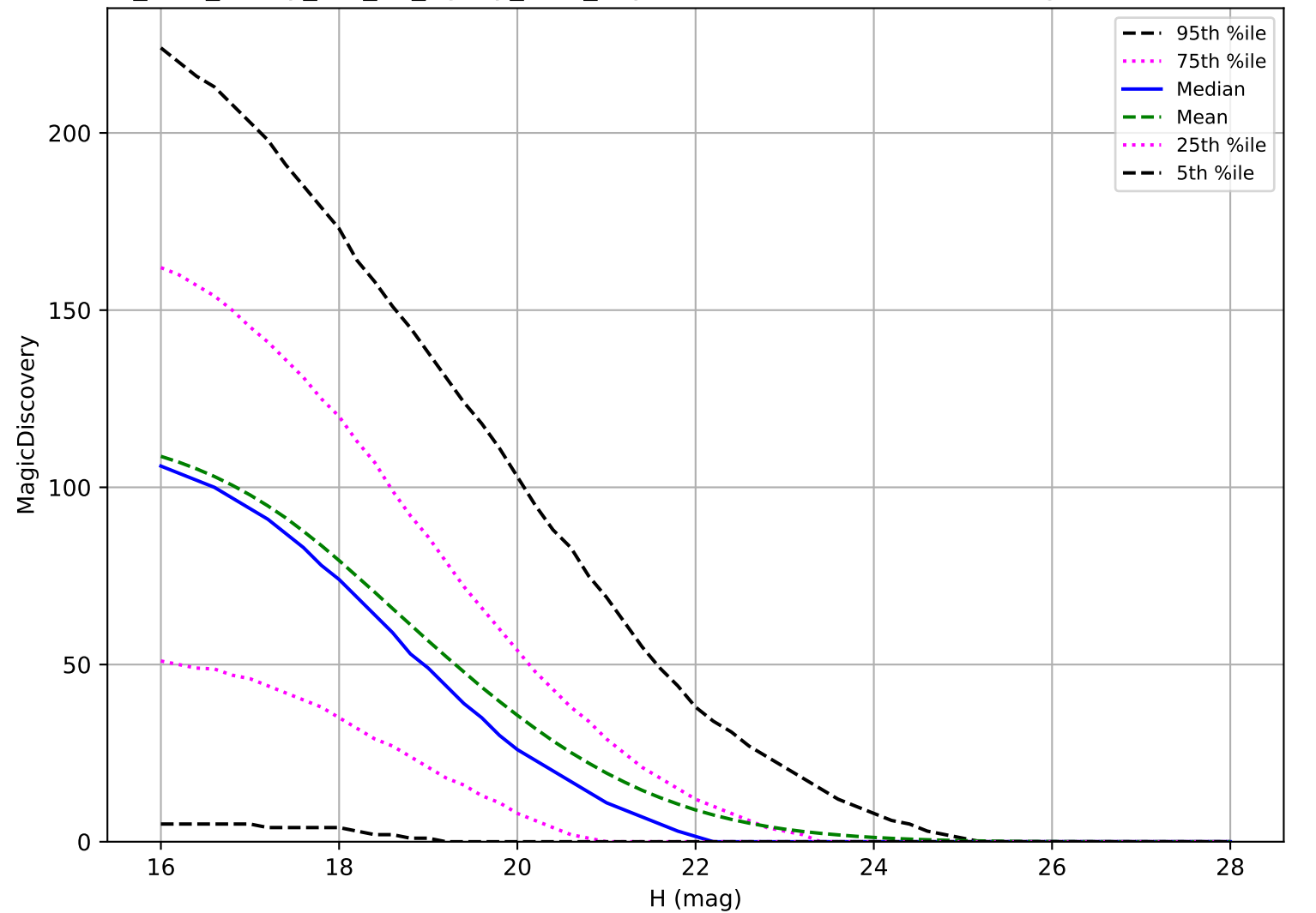
too_elab_heavy_r64_d2_ugrizy_v3.4_10yrs: NEO 6 detections in 60 nights detection loss
