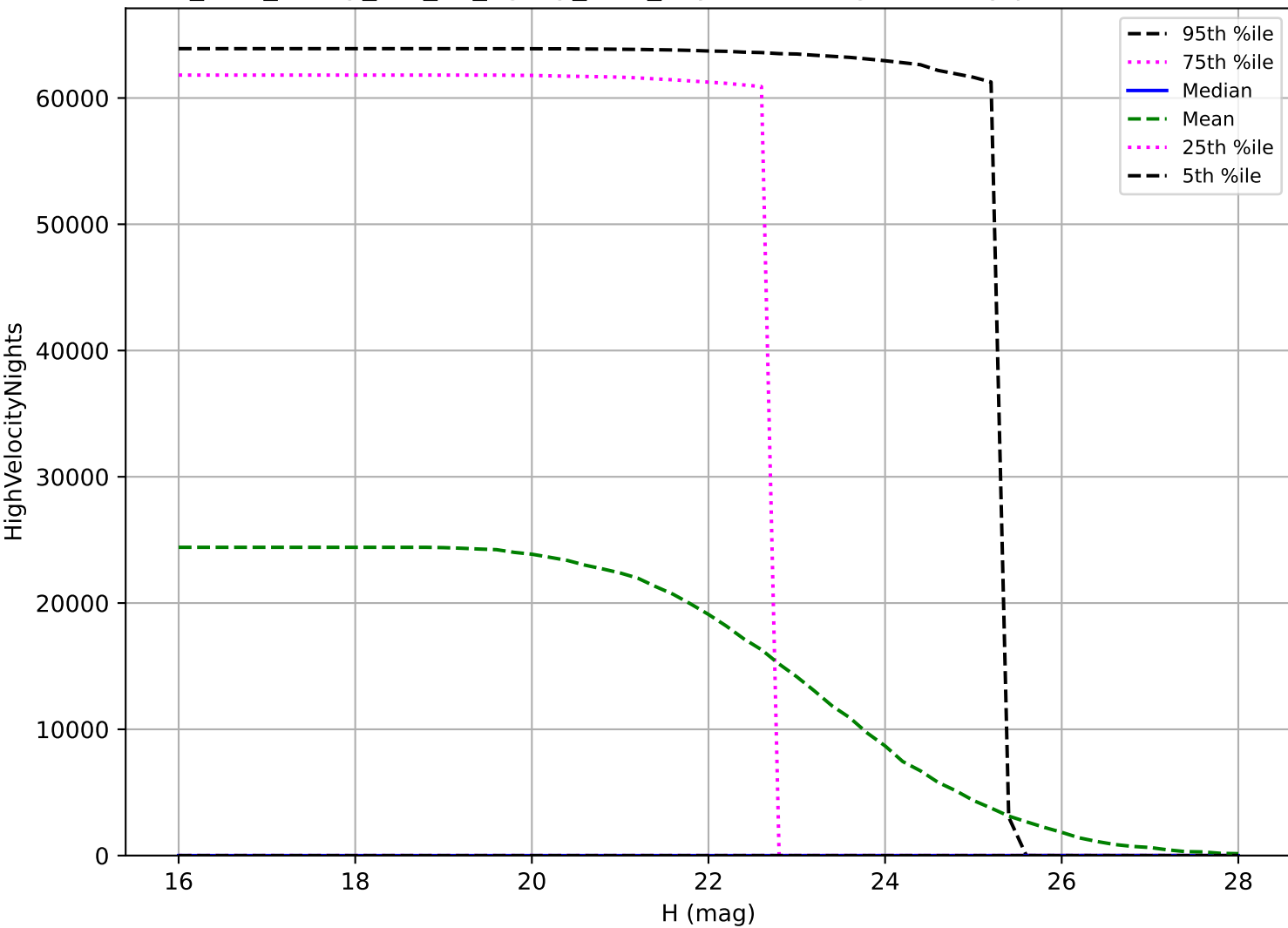
too_elab_heavy_r64_d2_ugrizy_v3.4_10yrs: PHA High velocity pair detection loss
