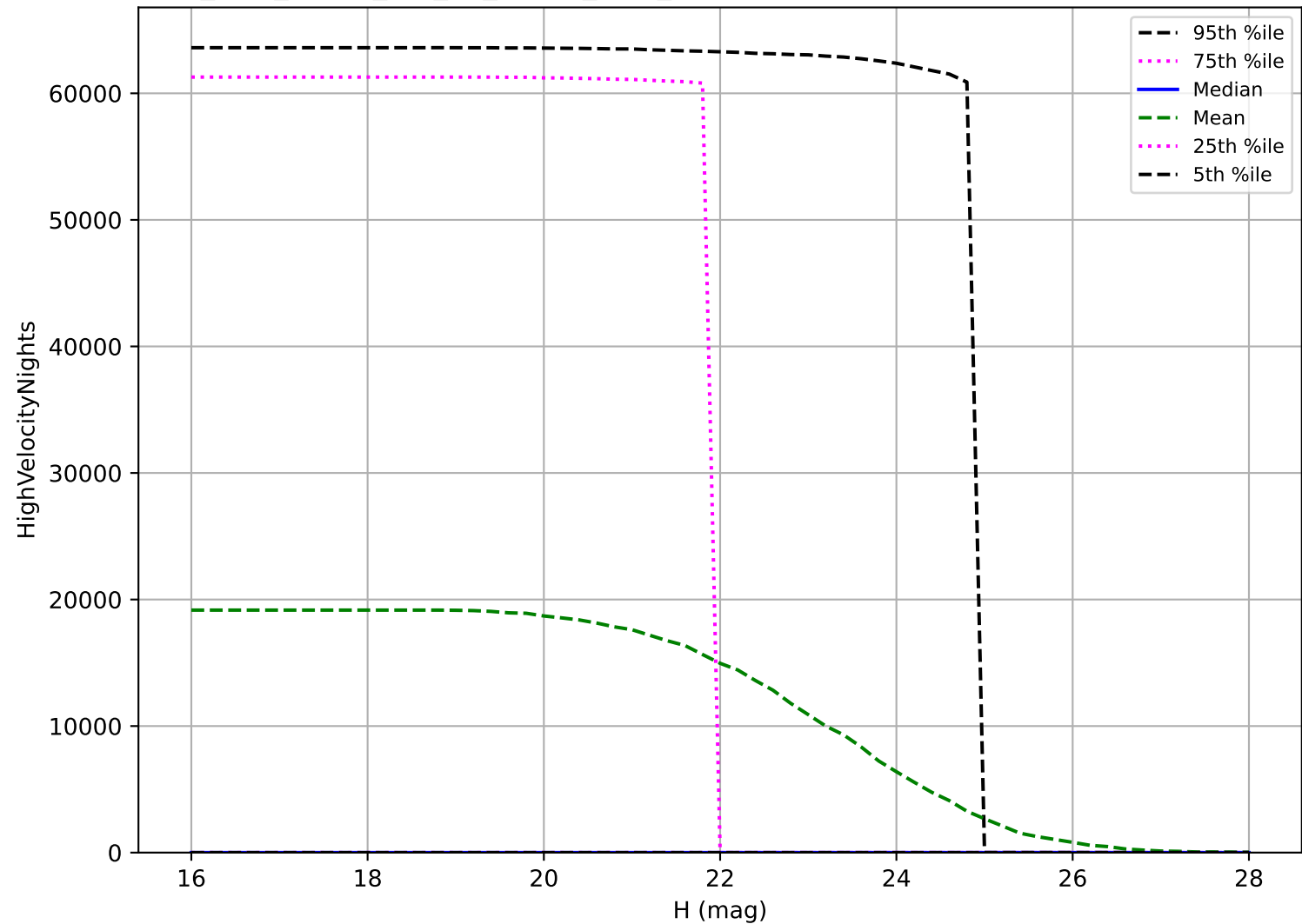
too_elab_heavy_r64_d2_ugrizy_v3.4_10yrs: NEO High velocity pair detection loss
