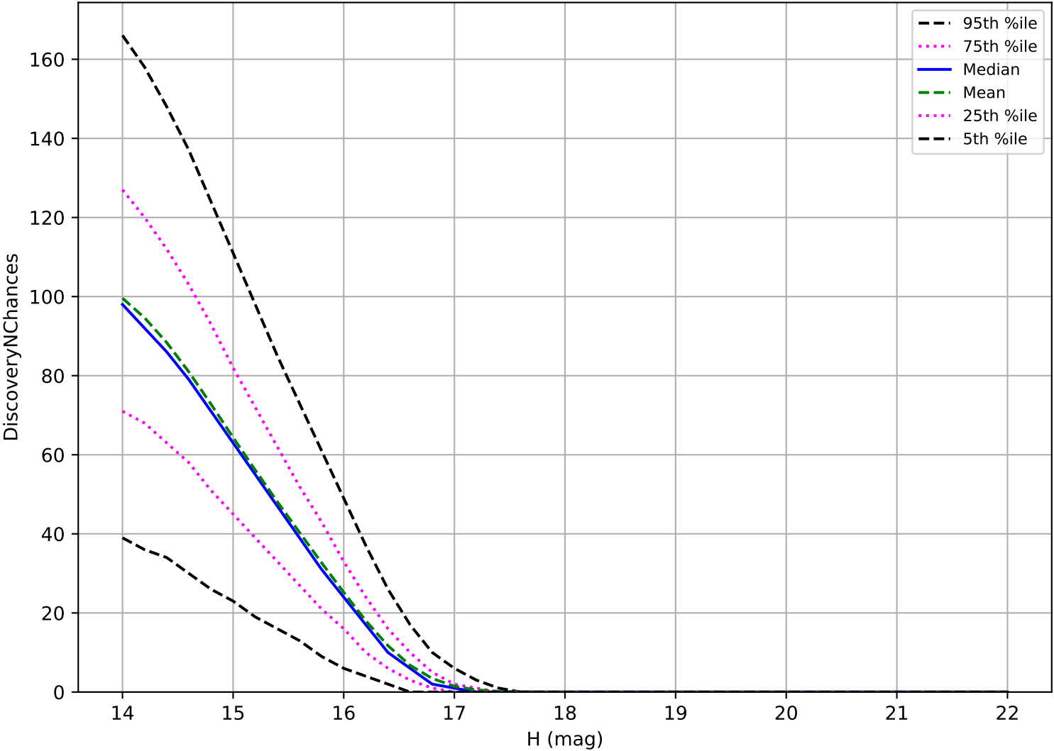
too_elab_heavy_r64_d2_ugrizy_v3.4_10yrs: Trojan 3 pairs in 15 nights detection loss
