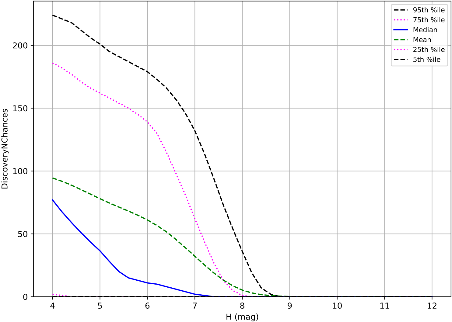
too_elab_heavy_r64_d2_ugrizy_v3.4_10yrs: TNO 3 pairs in 15 nights detection loss
