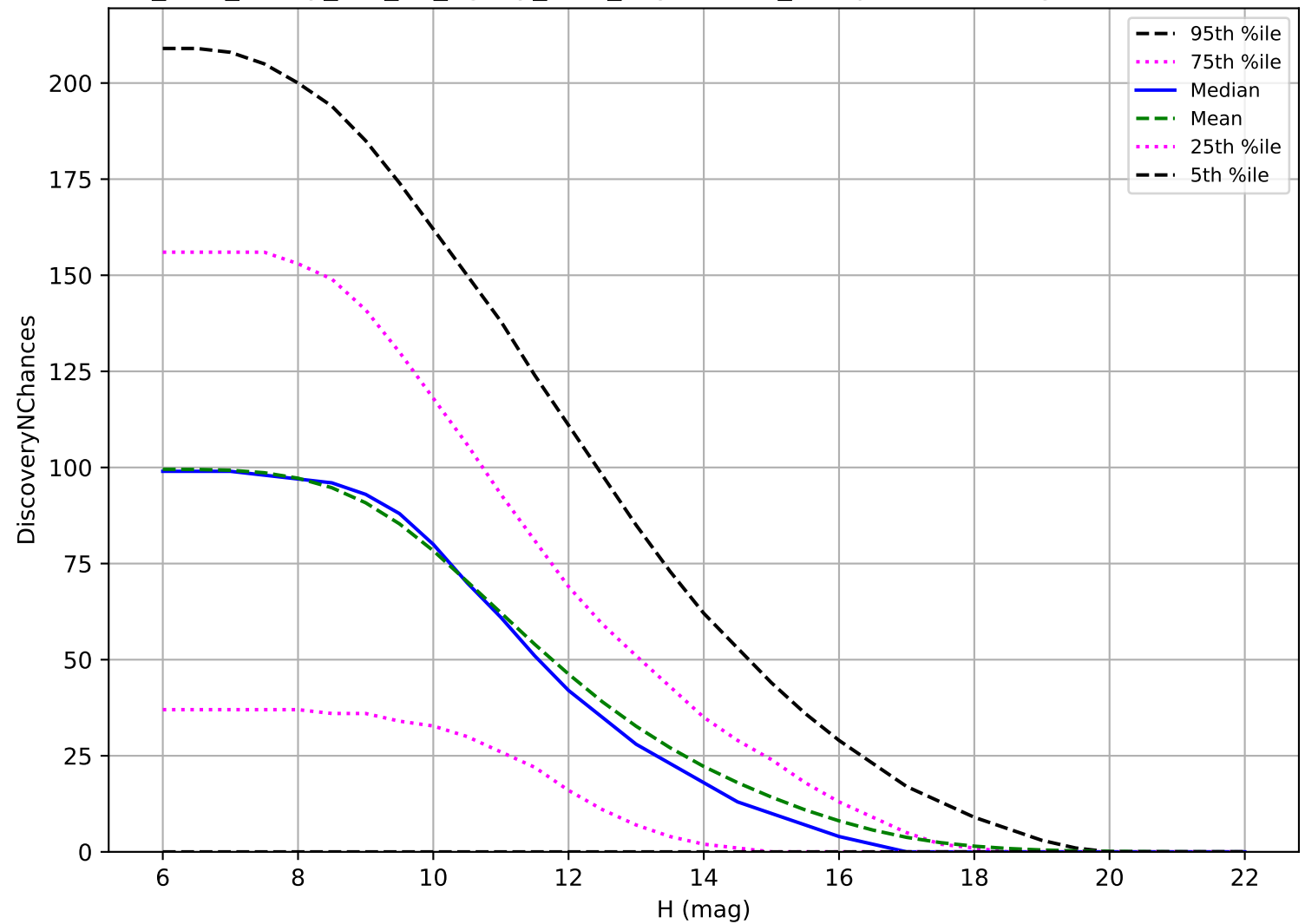
too_elab_heavy_r64_d2_ugrizy_v3.4_10yrs: OCC_r5 3 pairs in 15 nights detection loss
