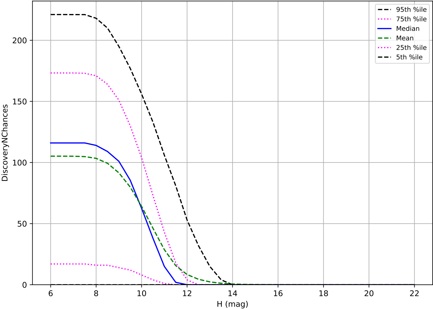
too_elab_heavy_r64_d2_ugrizy_v3.4_10yrs: OCC_r20 3 pairs in 15 nights detection loss
