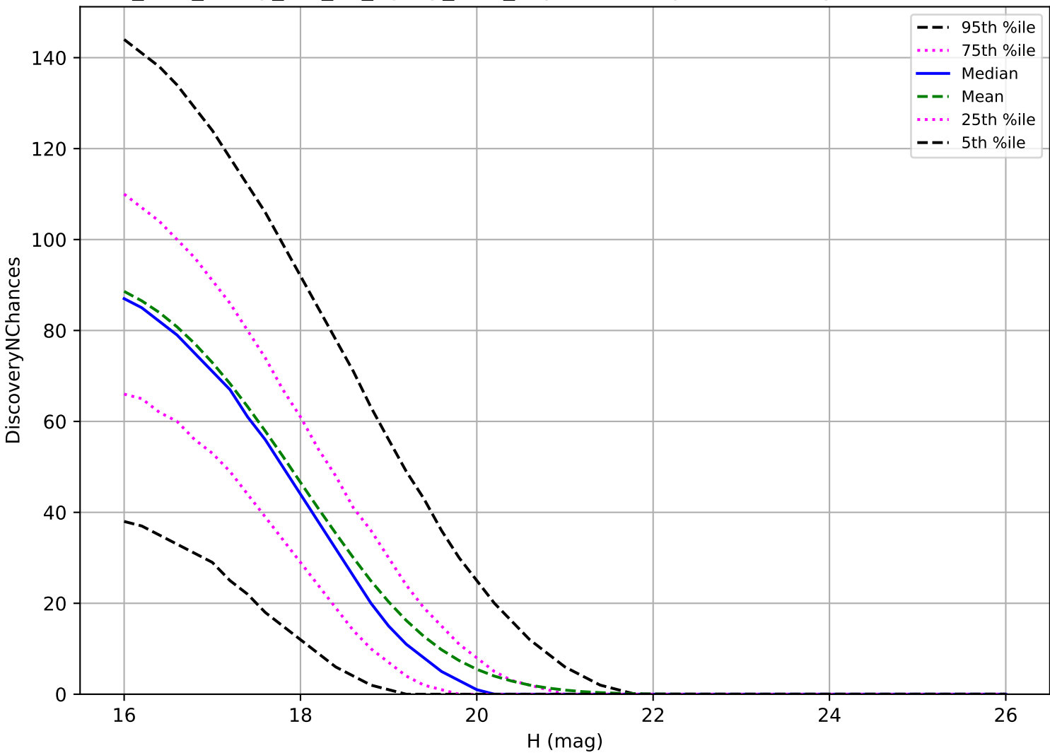
too_elab_heavy_r64_d2_ugrizy_v3.4_10yrs: MBA 3 pairs in 15 nights detection loss
