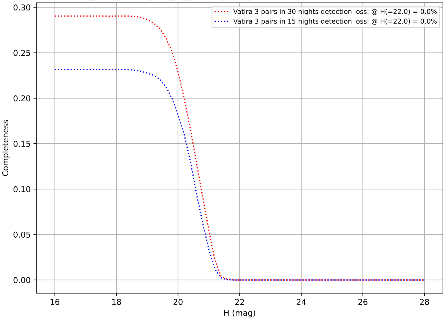
too_elab_heavy_r64_d2_ugrizy_v3.4_10yrs: DifferentialCompleteness
