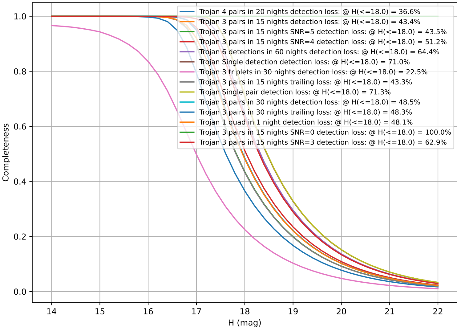
too_elab_heavy_r64_d2_ugrizy_v3.4_10yrs: CumulativeCompleteness
