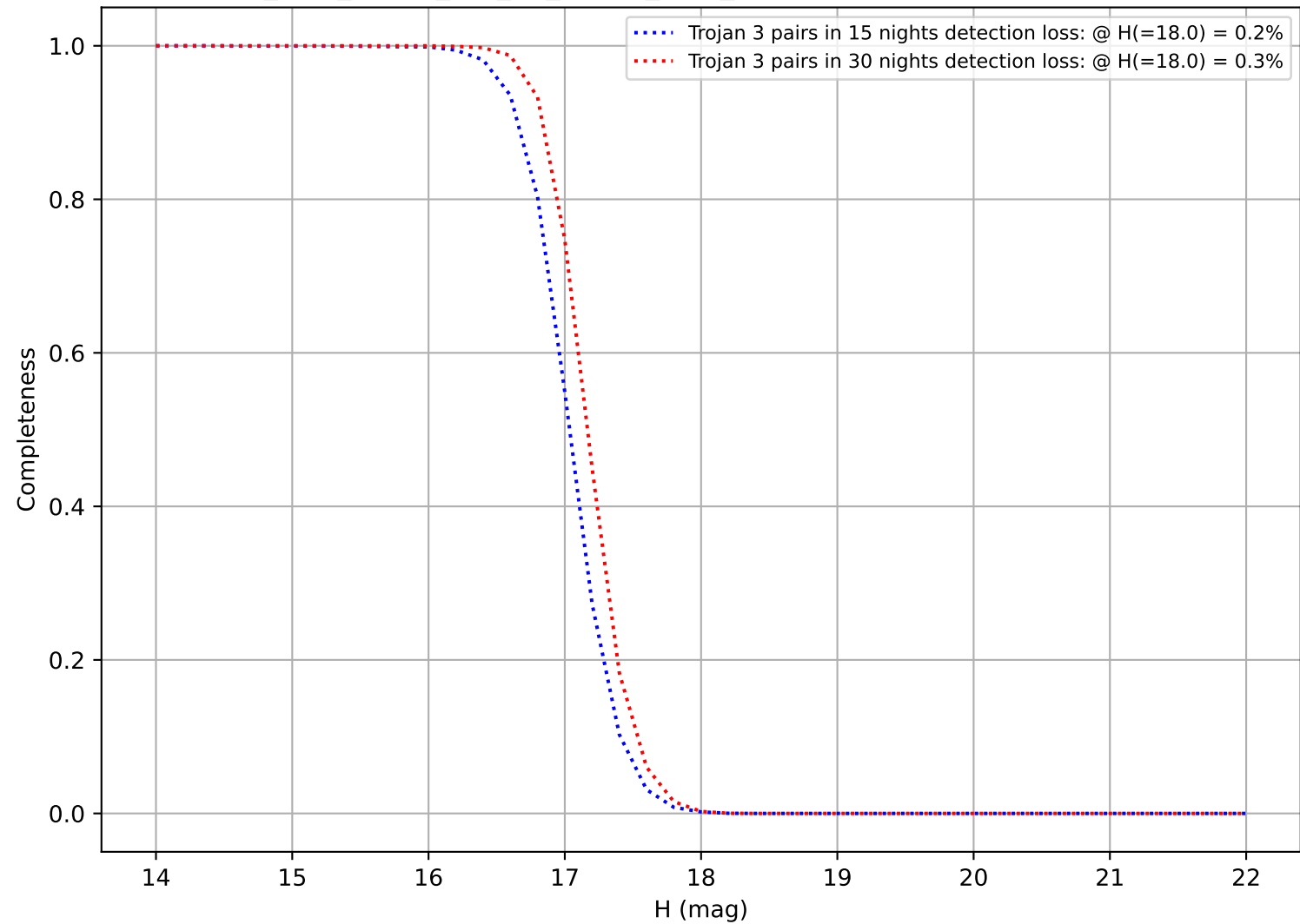
too_elab_heavy_r64_d2_ugrizy_v3.4_10yrs: DifferentialCompleteness
