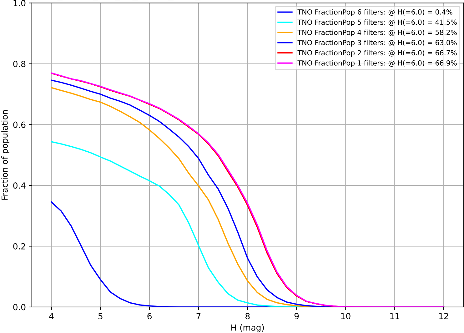
too_elab_heavy_r64_d2_ugrizy_v3.4_10yrs: Fraction of population with colors in X filters TNO
