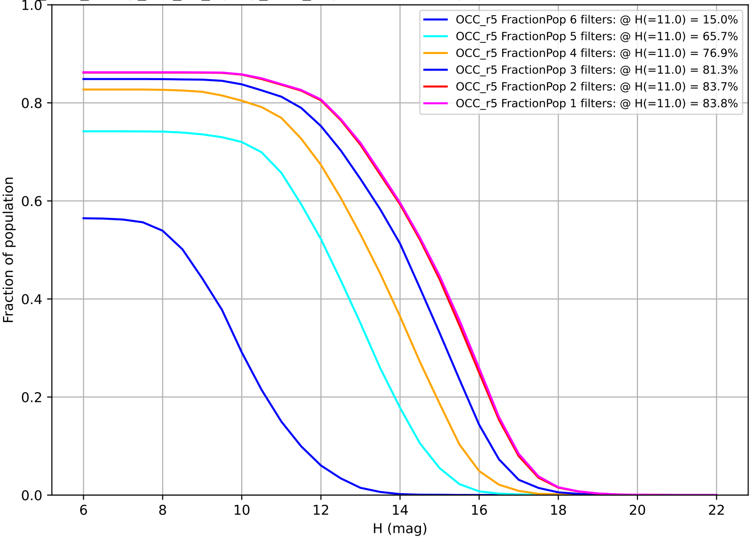
too_elab_heavy_r64_d2_ugrizy_v3.4_10yrs: Fraction of population with colors in X filters OCC_r5
