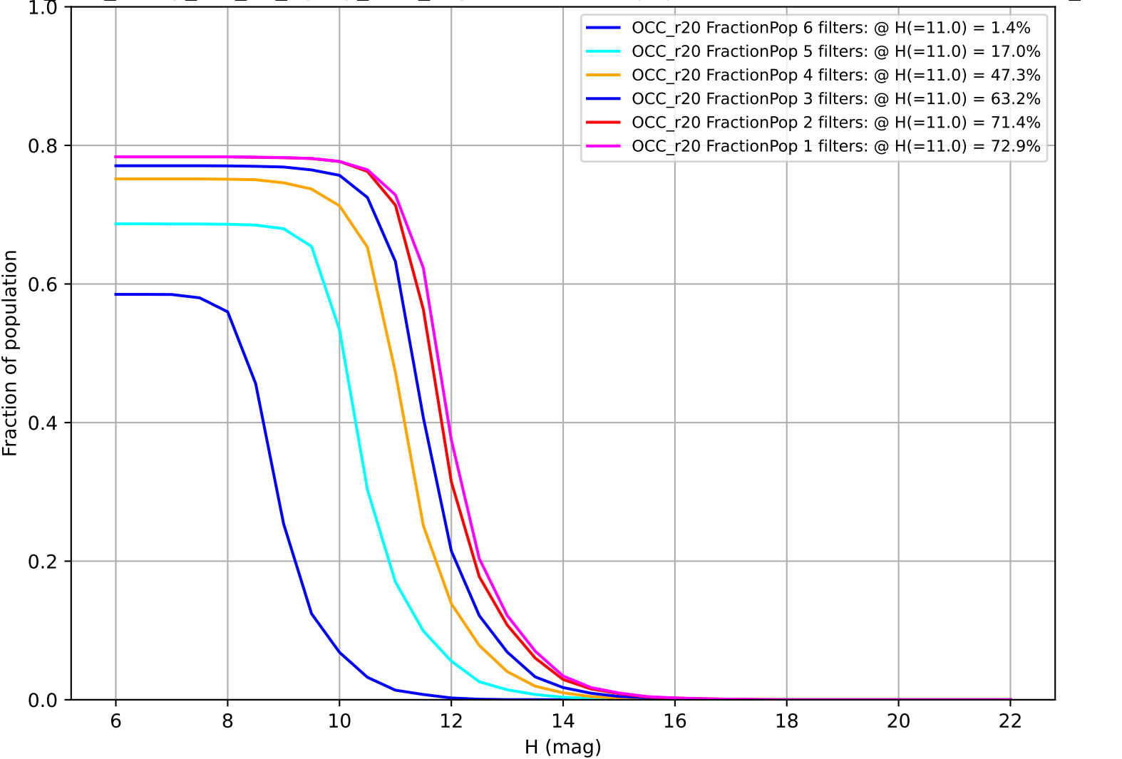
too_elab_heavy_r64_d2_ugrizy_v3.4_10yrs: Fraction of population with colors in X filters OCC_r20
