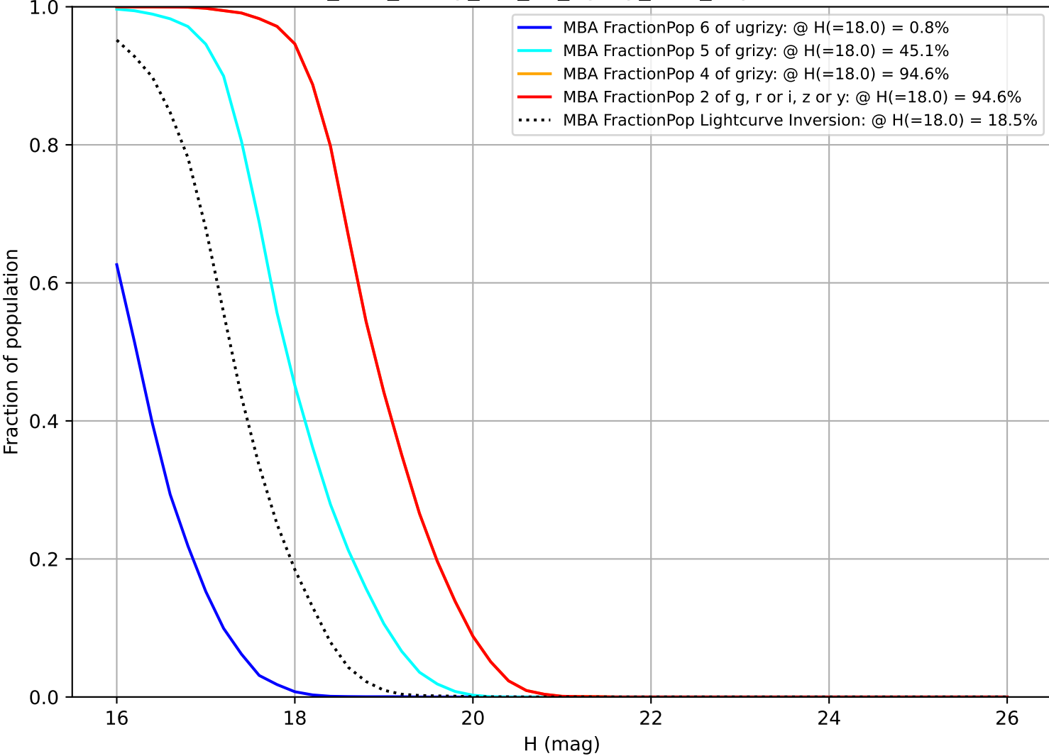
too_elab_heavy_r64_d2_ugrizy_v3.4_10yrs MBA
