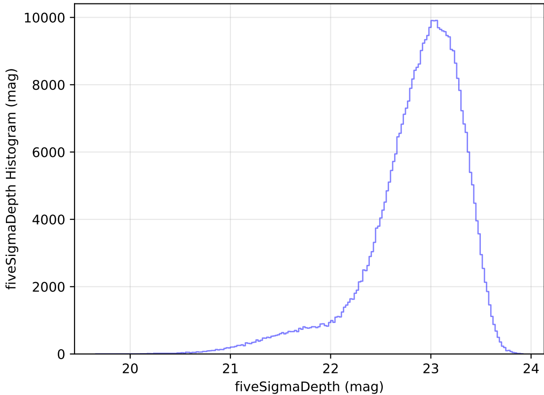
too_elab_heavy_r64_d2_ugrizy_v3.4_10yrs z: fiveSigmaDepth Histogram
