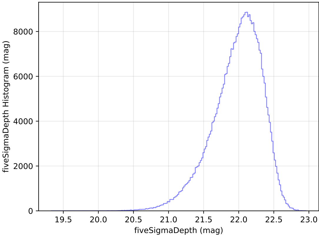
too_elab_heavy_r64_d2_ugrizy_v3.4_10yrs y: fiveSigmaDepth Histogram
