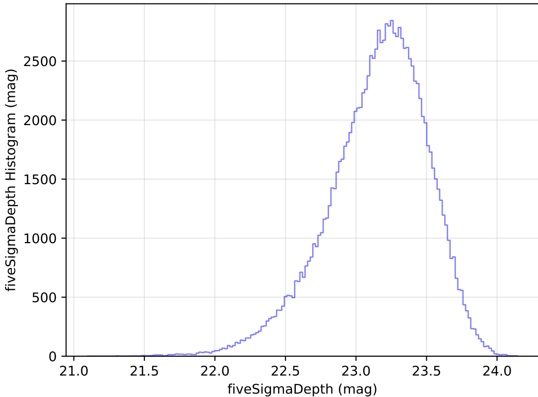
too_elab_heavy_r64_d2_ugrizy_v3.4_10yrs u: fiveSigmaDepth Histogram
