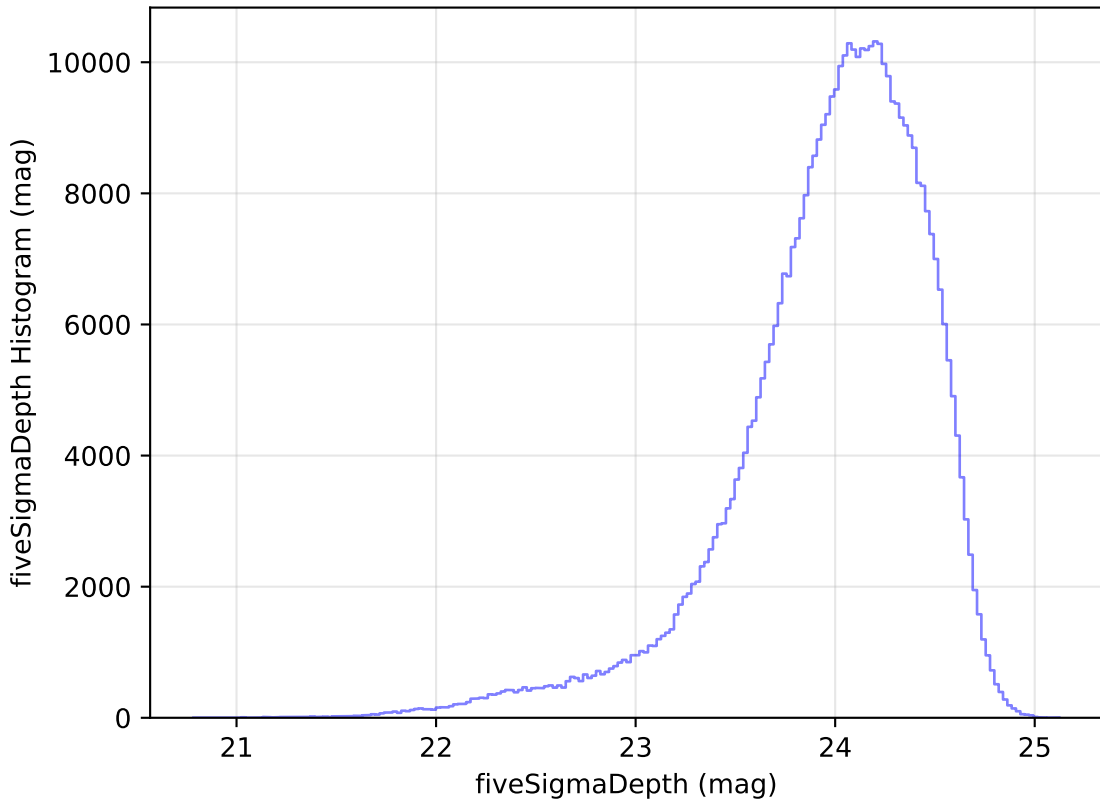
too_elab_heavy_r64_d2_ugrizy_v3.4_10yrs r: fiveSigmaDepth Histogram
