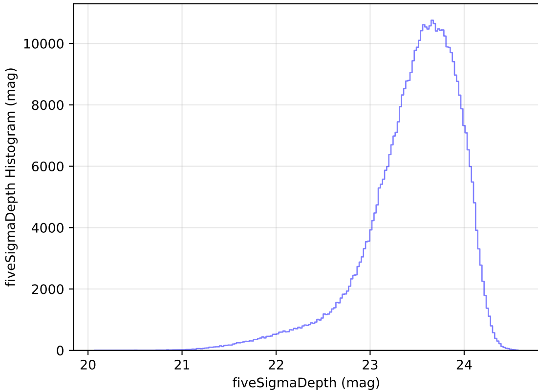
too_elab_heavy_r64_d2_ugrizy_v3.4_10yrs i: fiveSigmaDepth Histogram
