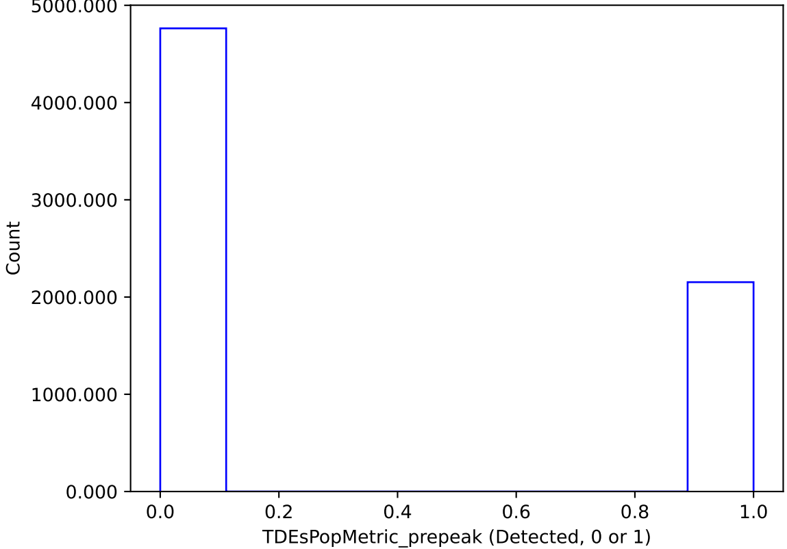
too_elab_heavy_r64_d2_ugrizy_v3.4_10yrs : TDEsPopMetric_prepeak
