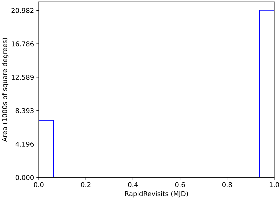
too_elab_heavy_r64_d2_ugrizy_v3.4_10yrs : RapidRevisits
