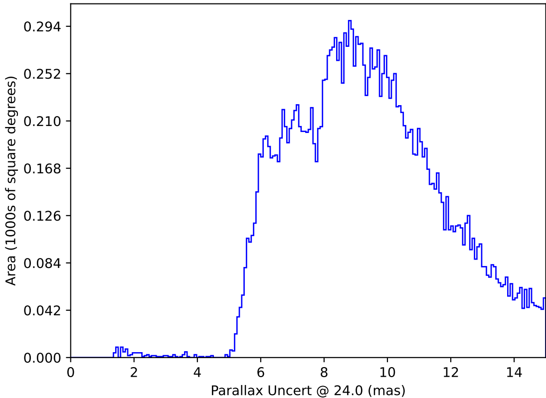
too_elab_heavy_r64_d2_ugrizy_v3.4_10yrs : Parallax Uncert @ 24.0
