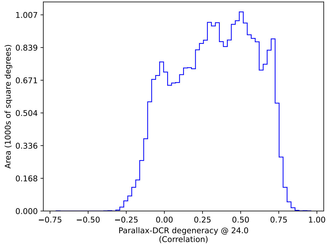
too_elab_heavy_r64_d2_ugrizy_v3.4_10yrs : Parallax-DCR degeneracy @ 24.0
