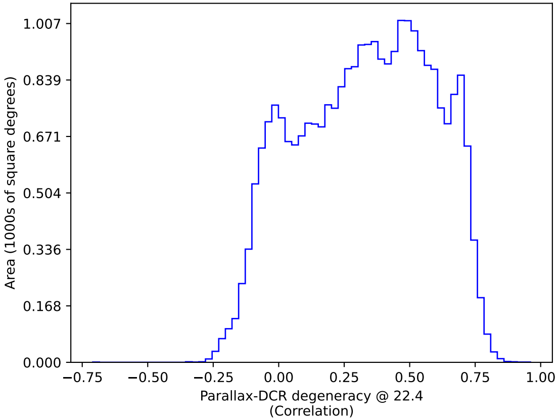
too_elab_heavy_r64_d2_ugrizy_v3.4_10yrs : Parallax-DCR degeneracy @ 22.4
