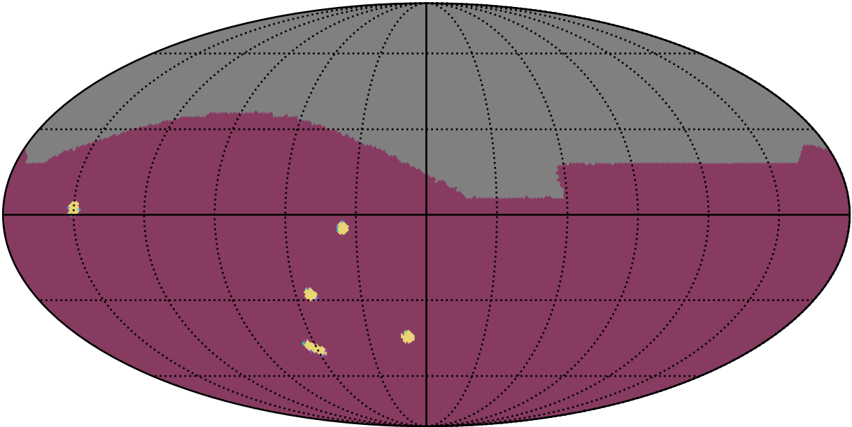
too_elab_heavy_r64_d2_ugrizy_v3.4_10yrs : NumberOfQuickRevisits
