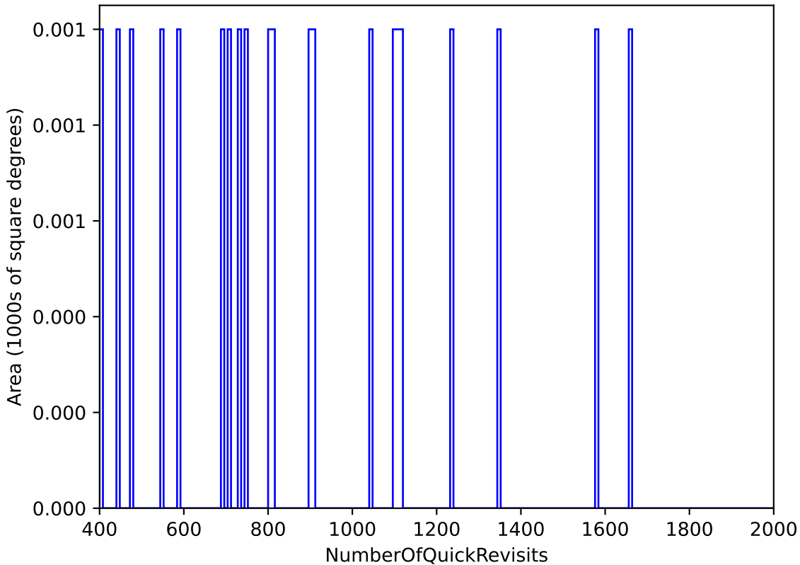
too_elab_heavy_r64_d2_ugrizy_v3.4_10yrs : NumberOfQuickRevisits
