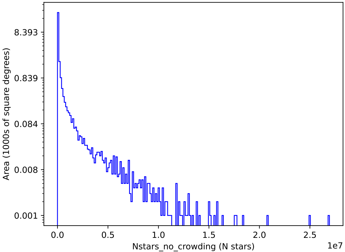
too_elab_heavy_r64_d2_ugrizy_v3.4_10yrs i: Nstars_no_crowding
