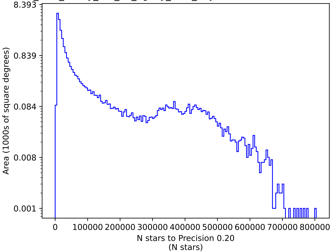
too_elab_heavy_r64_d2_ugrizy_v3.4_10yrs i: N stars to Precision 0.20
