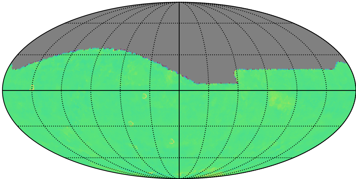
too_elab_heavy_r64_d2_ugrizy_v3.4_10yrs r: Kuiper rotTelPos
