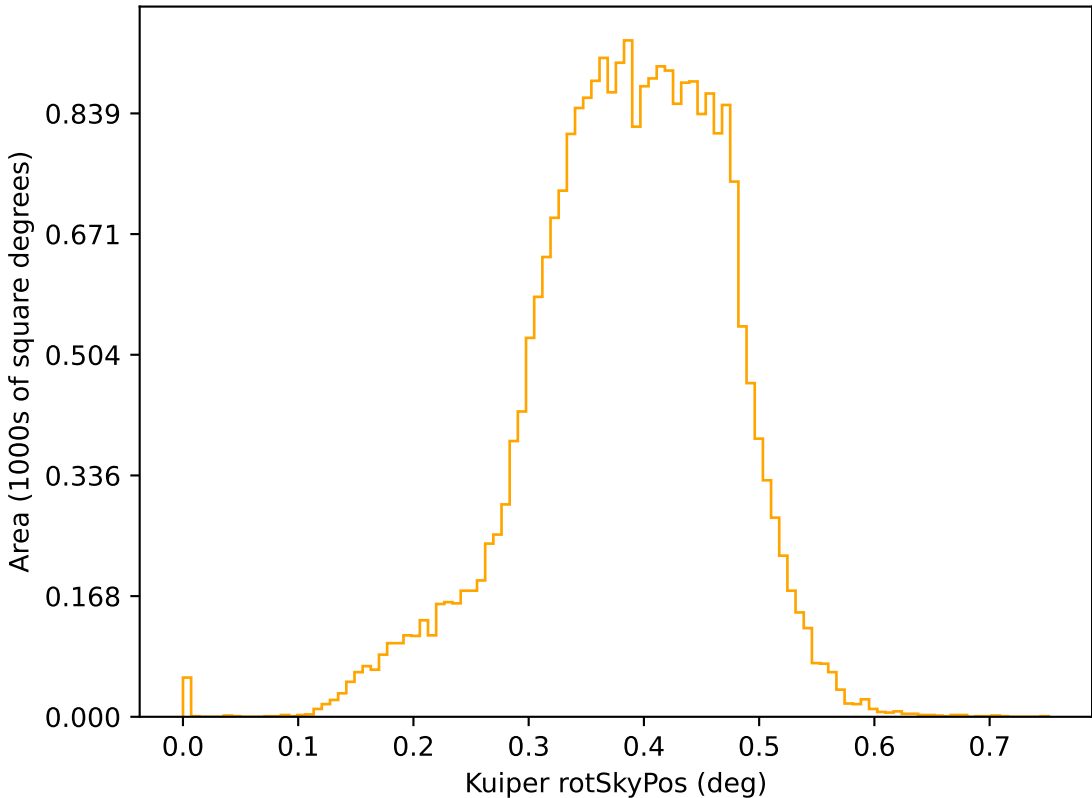
too_elab_heavy_r64_d2_ugrizy_v3.4_10yrs r: Kuiper rotSkyPos
