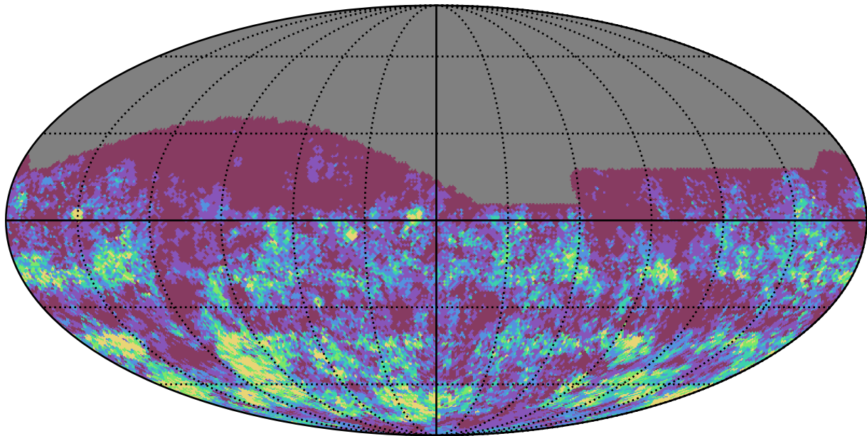
too_elab_heavy_r64_d2_ugrizy_v3.4_10yrs r band: Gaps_3hr
