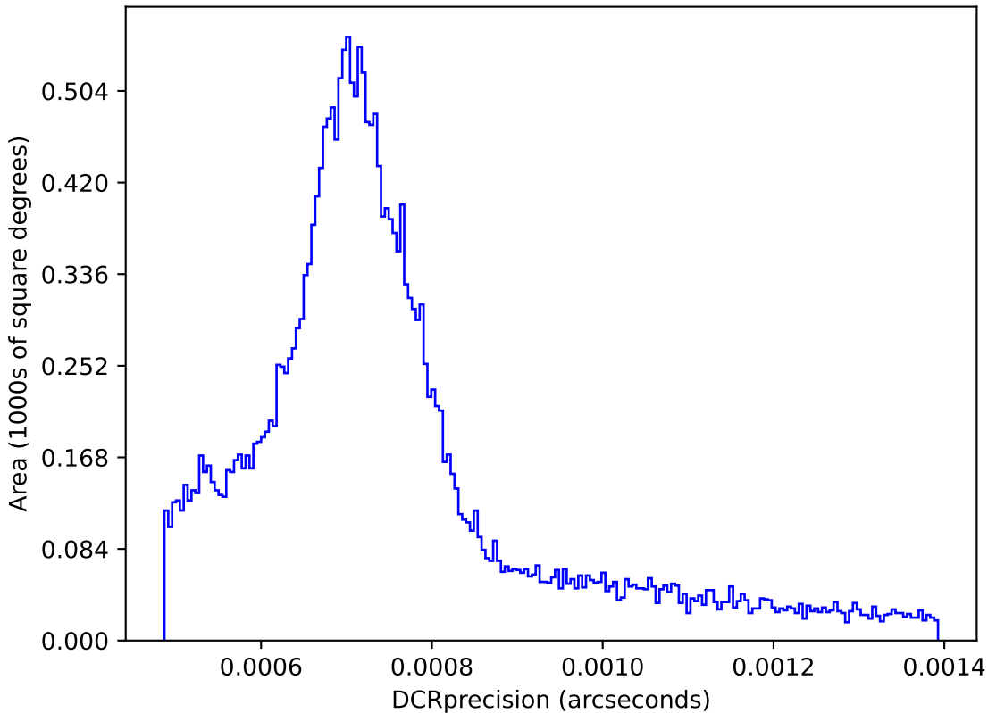
too_elab_heavy_r64_d2_ugrizy_v3.4_10yrs : DCRprecision
