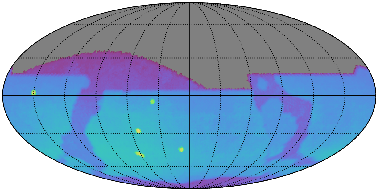
too_elab_heavy_r64_d2_ugrizy_v3.4_10yrs : Brown Dwarf, L7
