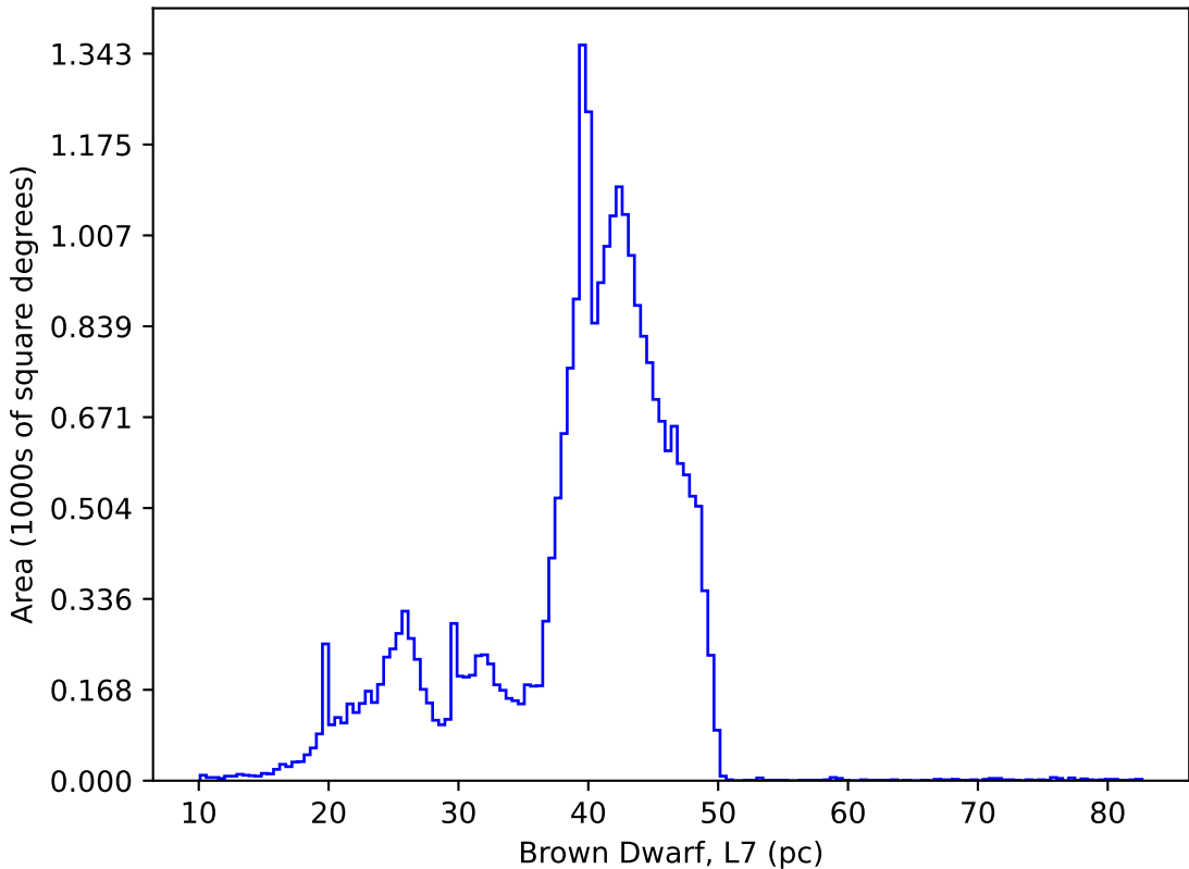
too_elab_heavy_r64_d2_ugrizy_v3.4_10yrs : Brown Dwarf, L7
