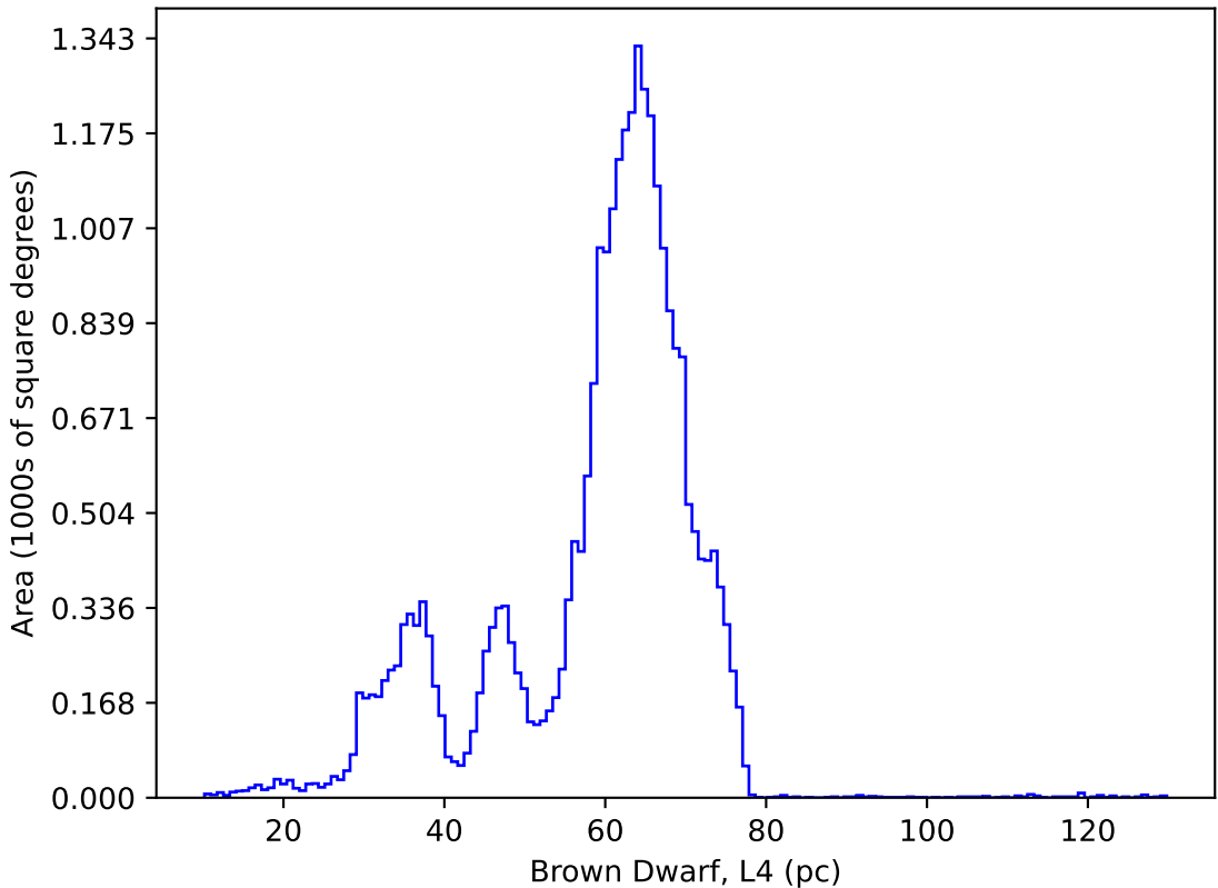
too_elab_heavy_r64_d2_ugrizy_v3.4_10yrs : Brown Dwarf, L4
