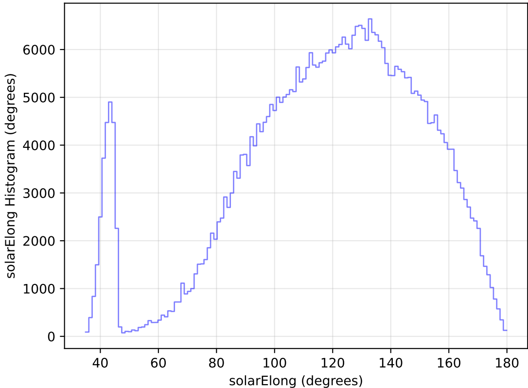
too_elab_heavy_r64_d2_ugrizy_v3.4_10yrs WFD z band: solarElong Histogram
