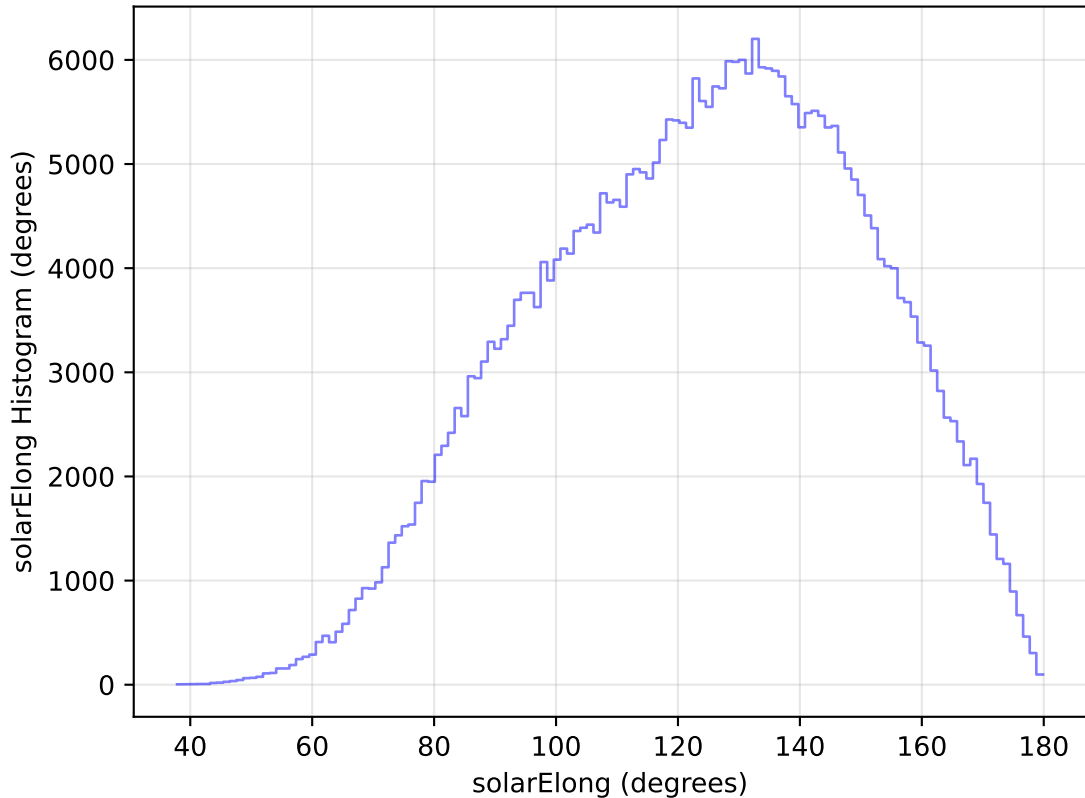
too_elab_heavy_r64_d2_ugrizy_v3.4_10yrs WFD y band: solarElong Histogram
