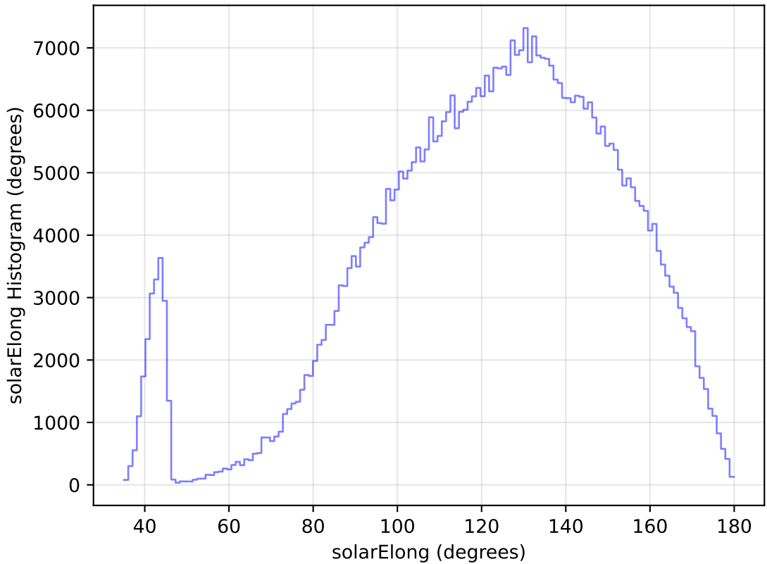
too_elab_heavy_r64_d2_ugrizy_v3.4_10yrs WFD i band: solarElong Histogram
