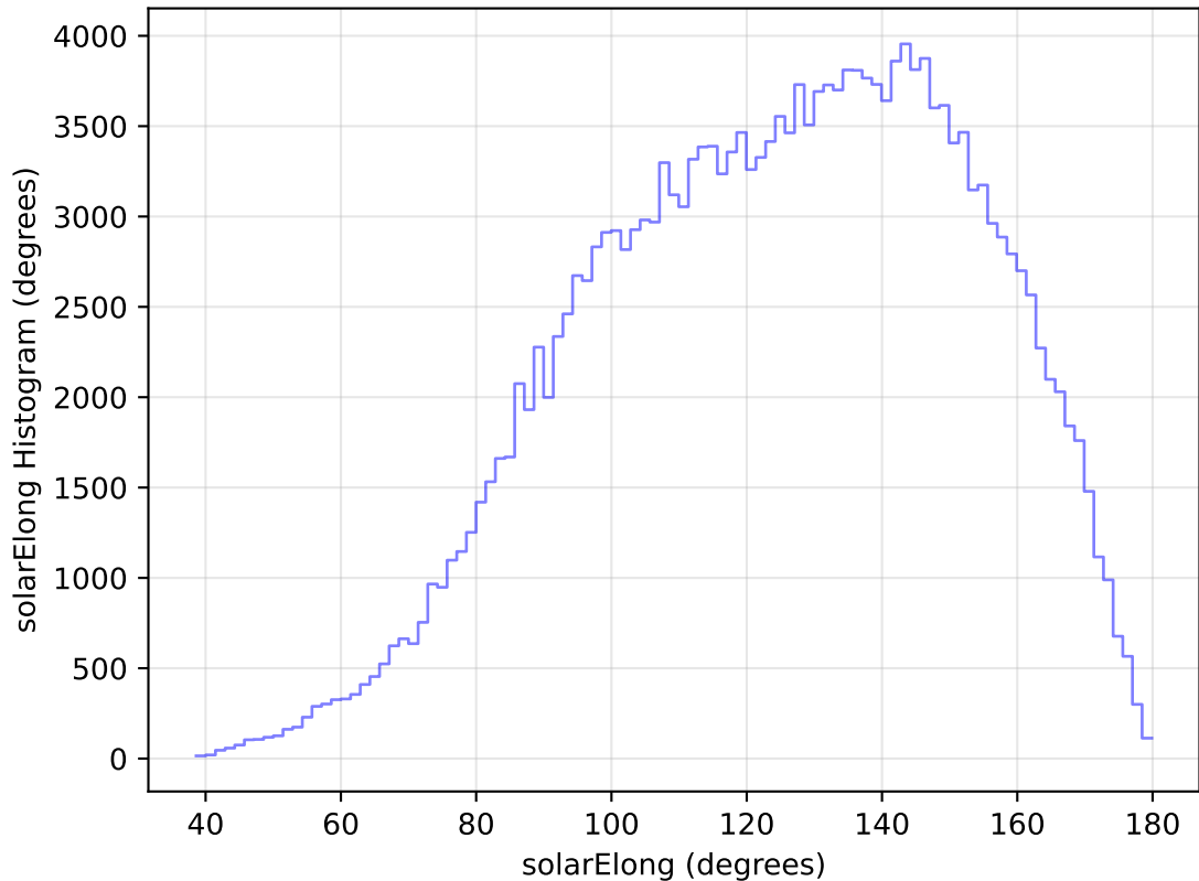
too_elab_heavy_r64_d2_ugrizy_v3.4_10yrs WFD g band: solarElong Histogram
