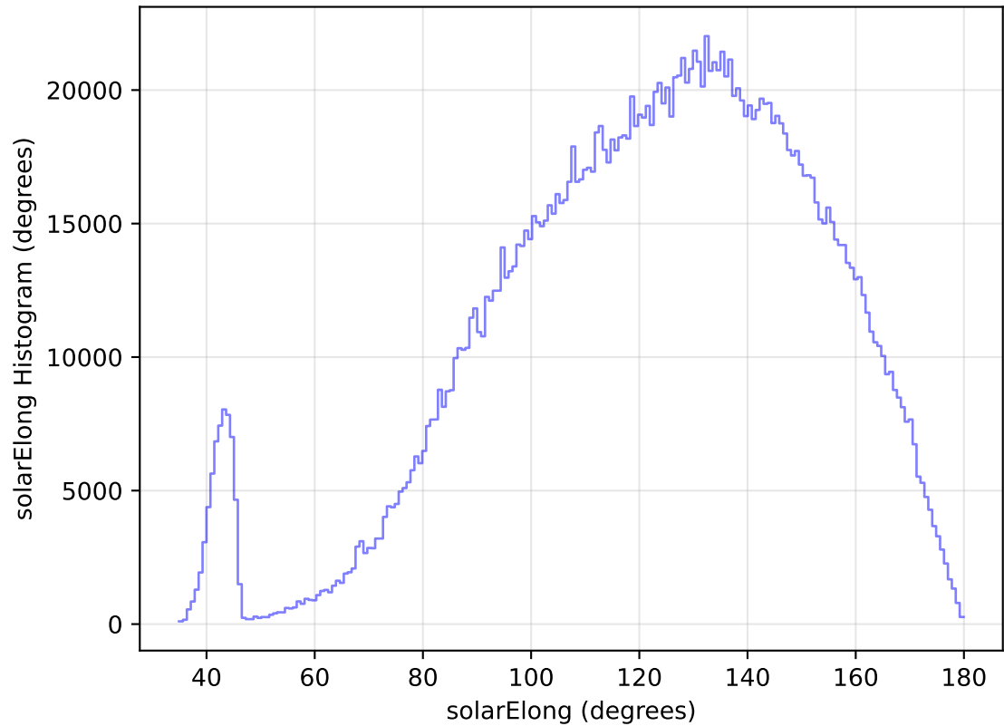
too_elab_heavy_r64_d2_ugrizy_v3.4_10yrs WFD all bands: solarElong Histogram
