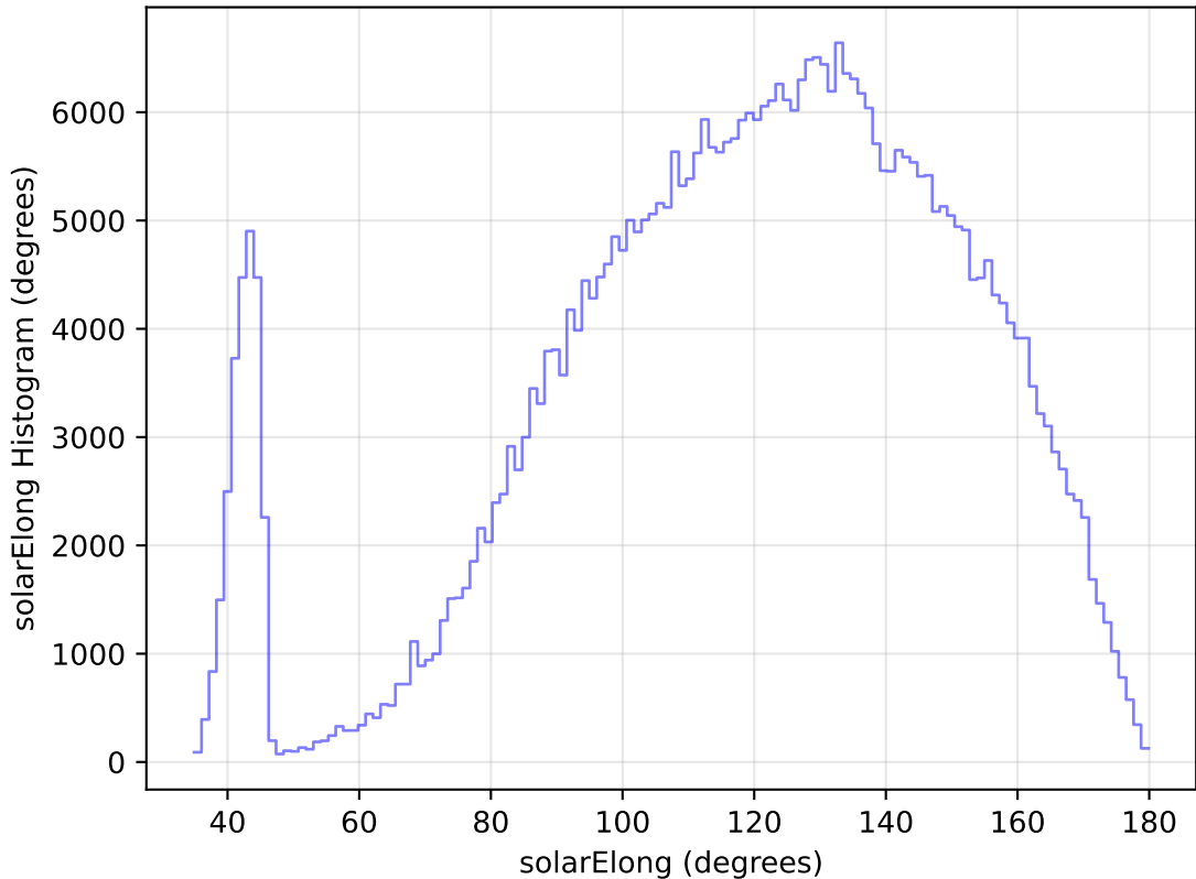
too_elab_heavy_r64_d2_ugrizy_v3.4_10yrs All sky z band: solarElong Histogram
