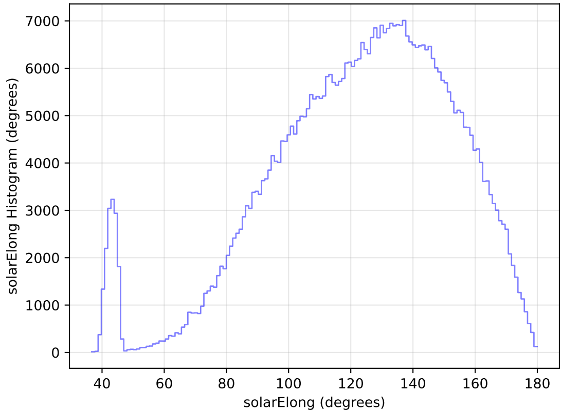
too_elab_heavy_r64_d2_ugrizy_v3.4_10yrs All sky r band: solarElong Histogram
